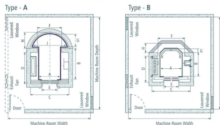
Hoistway Elevation Plan
