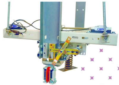
Car Frame Bottom Clutch
