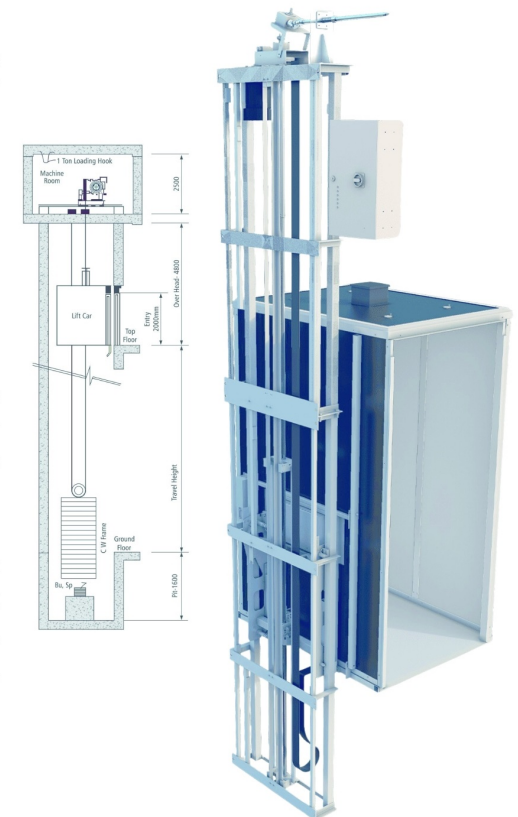
Lift car structure being sturdy and durable
